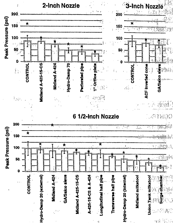
Figure 2. Effect of surge pressure reduction devices on peak pressure in 2-inch, 3-inch, and 6 1/2-inch safety vent nozzles.
